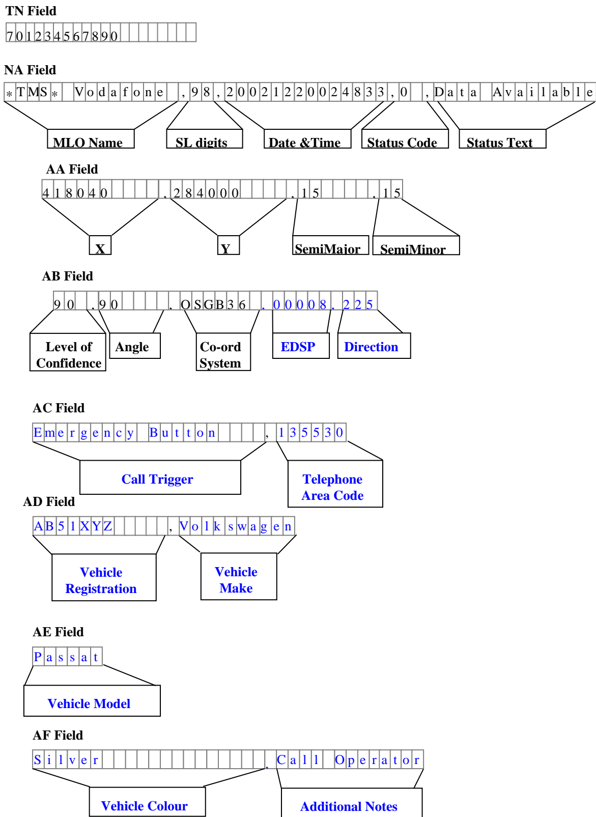
Figure 5 QP PDU Field Format for Telematics “Data Available” Message
