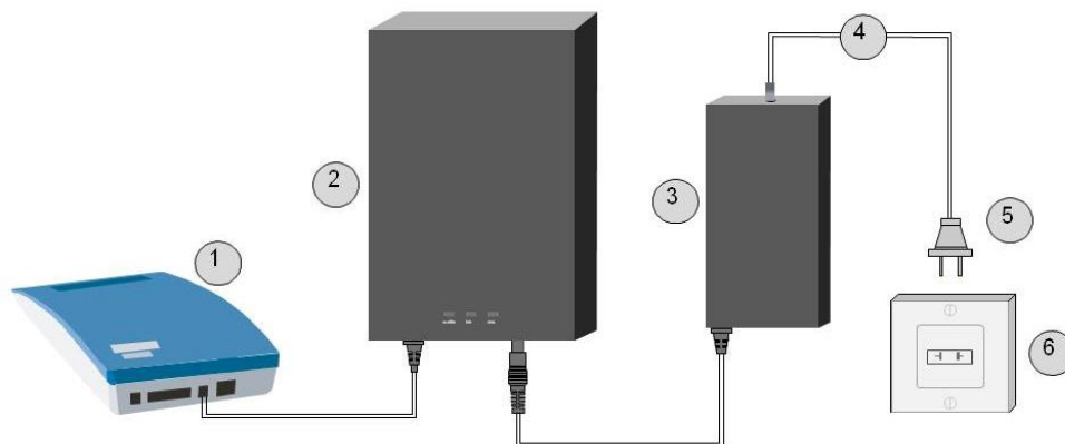
Legend: 1-ONT; 2-BBU; 3-Charger/Adaptor; 4/5- AC Power Cable & Plug; 6-Power Socket
