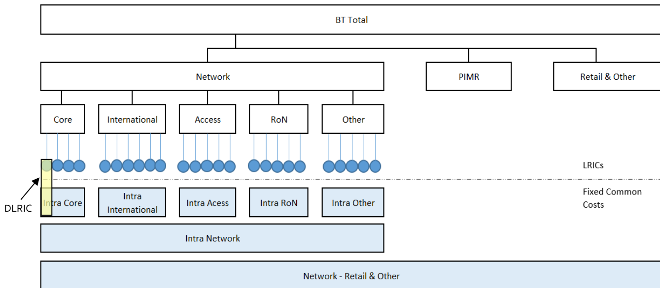
Figure 3.14 DLRIC Calculation
